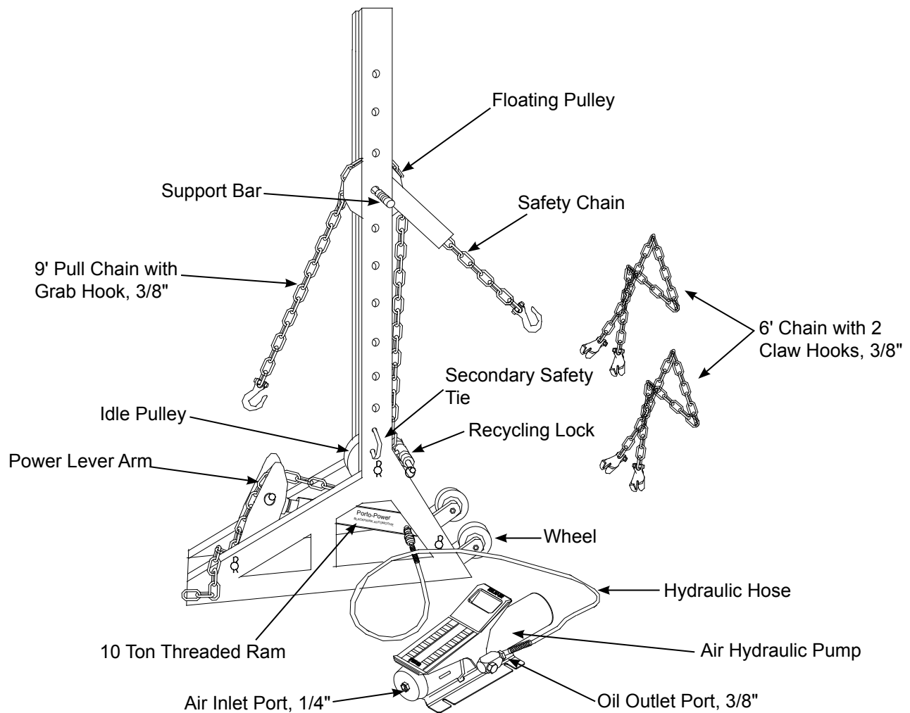
Figure 1 - B93601B Components
