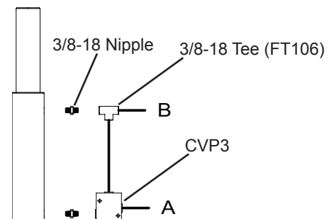
Figure 2 - Double-acting cylinder configuration.
