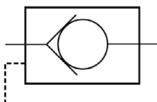
Figure 1 - Switch is wired normally open and held closed by spring force.
